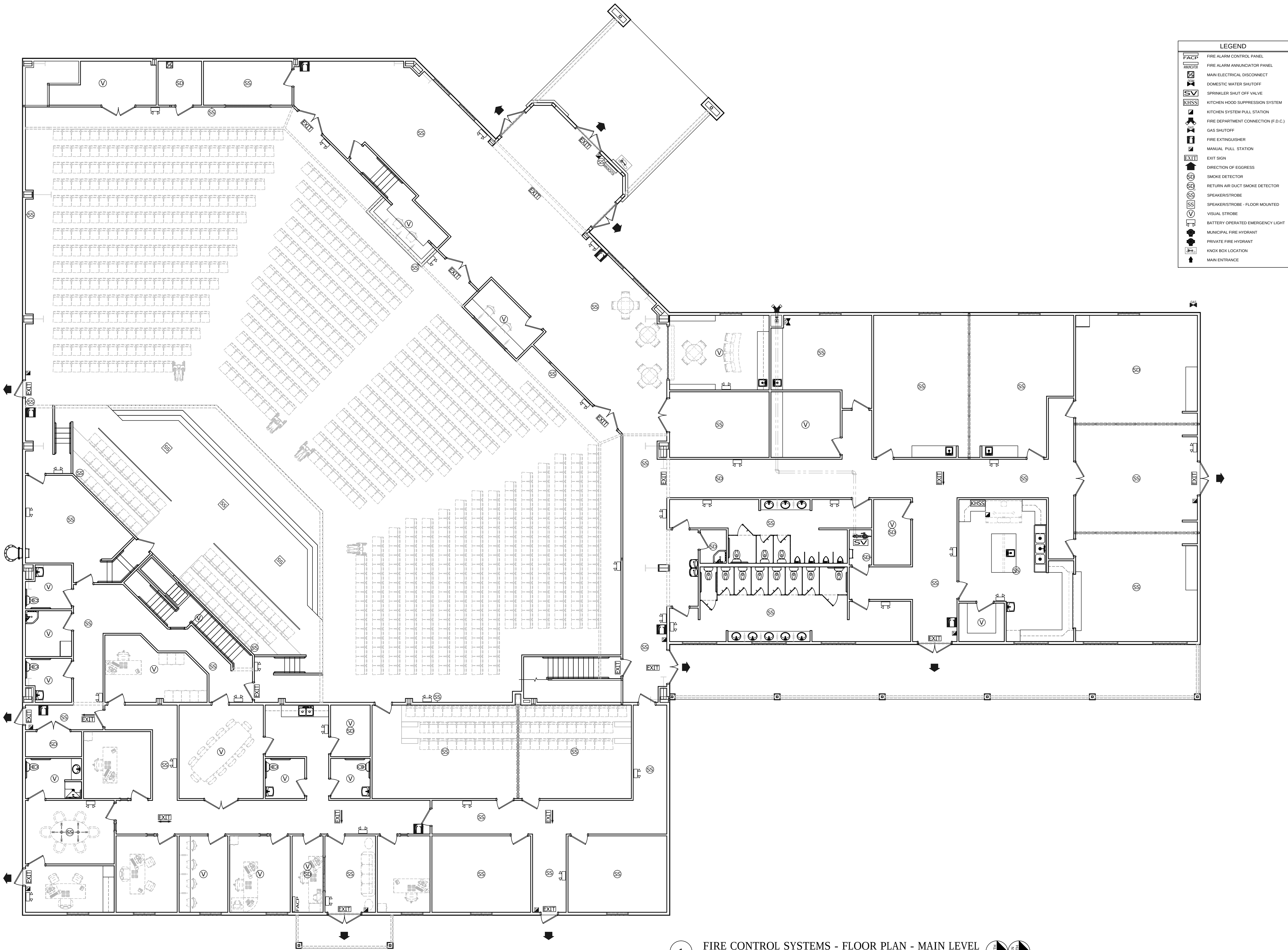
1 FIRE CONTROL SYSTEMS - FLOOR PLAN - MAIN LEVEL Scale: 1/8" = 1'
