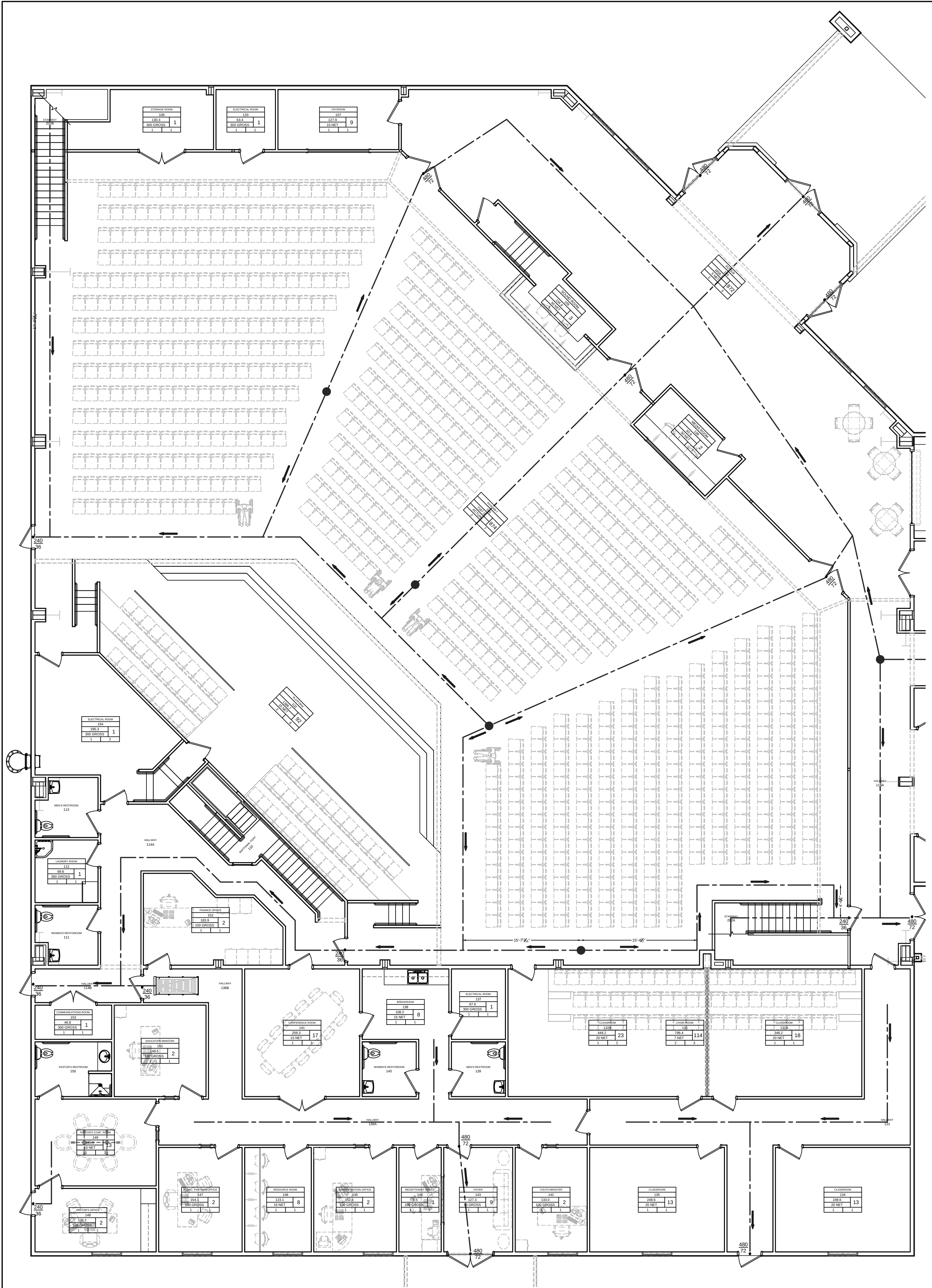
1 FIRE EGRESS INFORMATION - FLOOR PLAN - MAIN LEVEL (ALT. 1)
