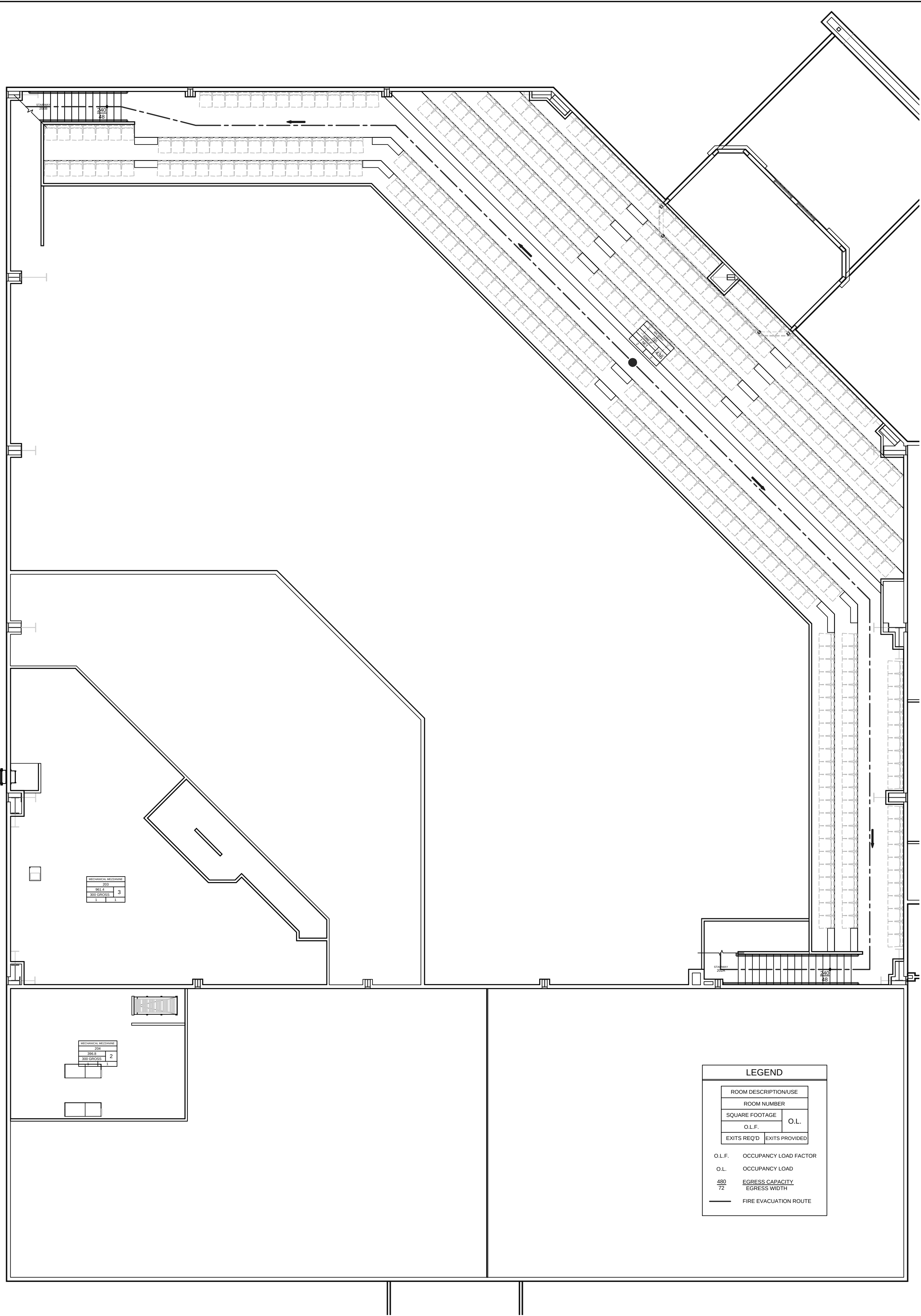
2 FIRE EGRESS INFORMATION - FLOOR PLAN - UPPER LEVEL (ALT. 1)
